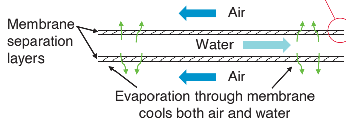
heat exchanger
